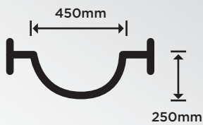
Trough Section
